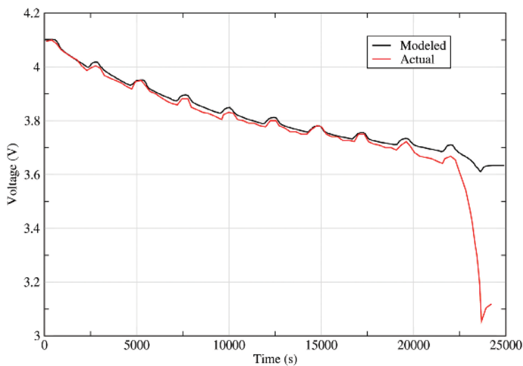
This example discharge model shows recovery charge when the load is disconnected. This matches experimental results very closely. Test data courtesy A&D Technologies, Michigan.
