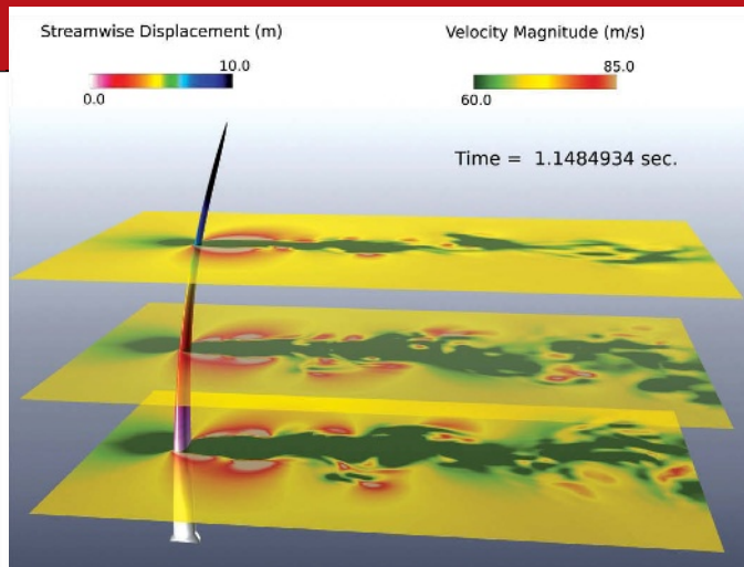
A direct coupled fluid-structure interaction simulation of a 100m composite blade, using Altair HyperWorks for calculating turbine blade aeroelasticity. Displayed are flow features at different cut planes. Image courtesy Altair Engineering.
