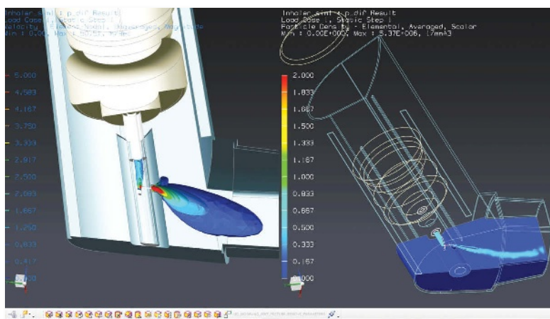
Multiphysics flow simulation of a medical inhaler, performed with NX CAE software from Siemens PLM Software. Image courtesy Siemens PLM Software.
