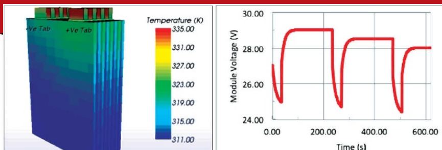
FIGURE 2: Simulation results for an eight-cell module; temperature is shown on the left and overall module response is shown on the right.
