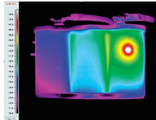
This IR image shows internal damage or a “soft short” in a lead acid battery. The damage is not visible when inspecting the battery.
