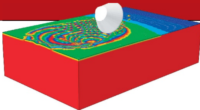
Dynamics of a re-entry vehicle impacting water at 30 ft./sec. The simulation consists of one structure (the capsule) and two fluids (air and water) whose interactions are captured in a single Abaqus FE model using the Coupled Eulerian-Lagrangian (CEL) technique to handle the highly discontinuous contact and free surface conditions. Image courtesy SIMULIA.
