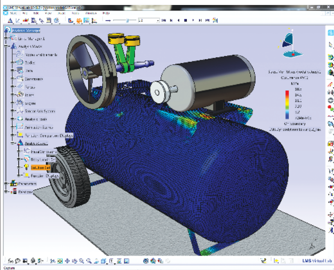
FIGURE 5: LMS Virtual.Lab simulation of a compressor, integrating engine motion, deformation, acoustics, fatigue and optimization computations.
