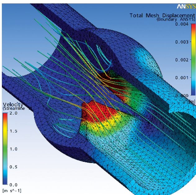
ANSYS software analysis of fluid-structure multiphysics interaction in a biomedical valve, taking into account strongly coupled fluid flow and structural deformations. Image courtesy ANSYS.
