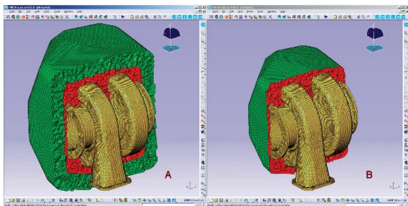
FIGURE 3: AML technology (B) allows LMS Virtual.Lab Acoustics to achieve higher-frequency resolution with a smaller mesh compared to PML (A).
