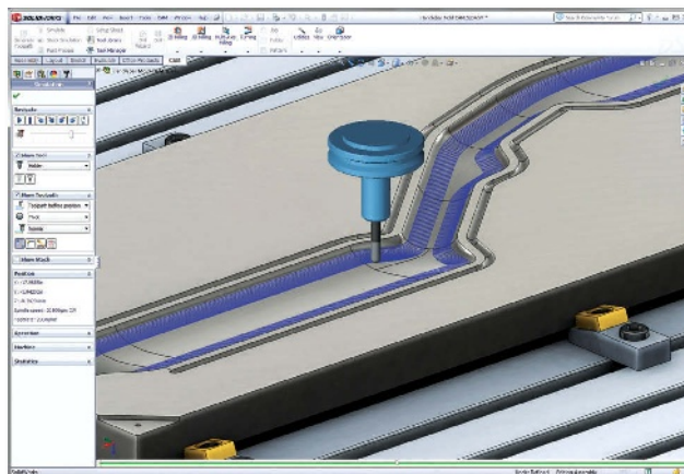
Working on a handlebar in HSMWorks.
