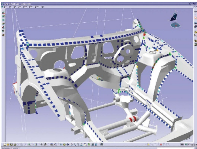
FIGURE 4: Seam welds are detected automatically in LMS Virtual.Lab Durability.
