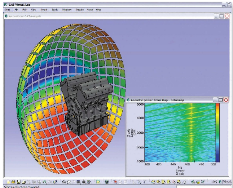
FIGURE 1: Sound Power radiation plot and color map for an engine run-up event.
