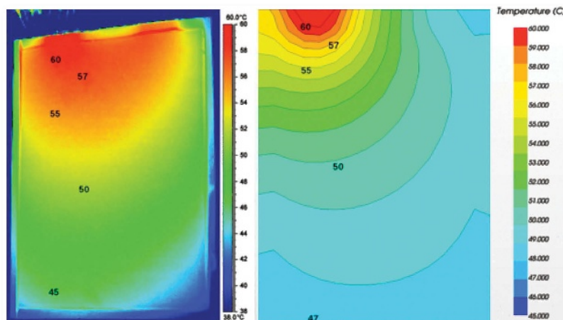
FIGURE 1: Comparison of simulated results (right side), with previously reported IR temperature measurements 4 .
