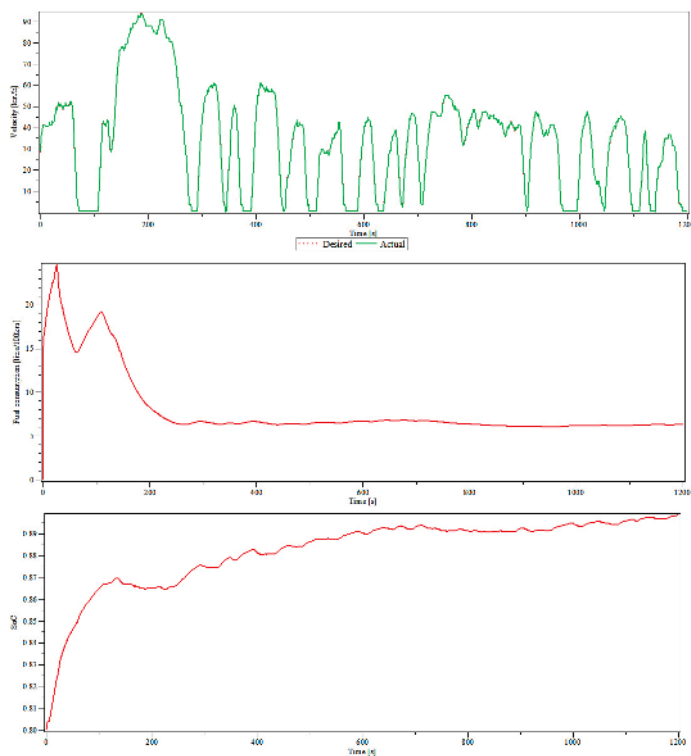
Results from full-vehicle HEV test using an urban drive cycle. The battery state-of-charge and fuel consumption are shown.
