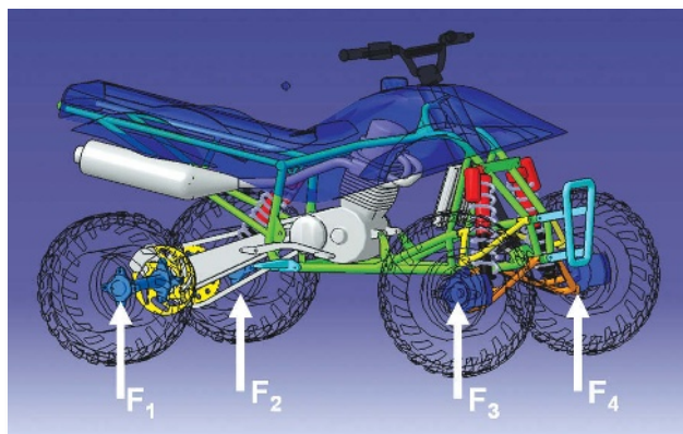
FIGURE 2: LMS Virtual.Lab Motion TWR replaces tires with actual measured road loads.
